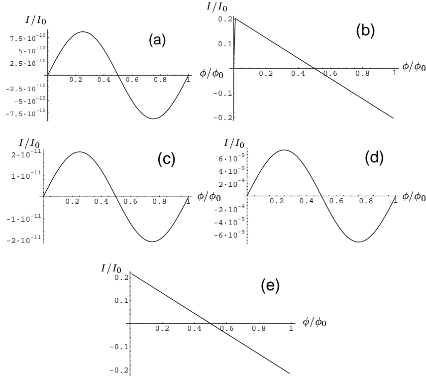
Fig. 5. The examples of normalised persistent currents \frac{I}{I_0} versus \frac{\phi}{\phi_0} in tori made with nanotubes of different chiralities, with approximately the same length and twist. The tori whose currents are presented here are (a) (4, 0) \times (-30, 60) , (b) (4, 1) \times (-39, 60) , (c) (4, 2) \times (-44, 55) , (d) (4, 3) \times (-51, 55) and (e) (4, 4) \times (-50, 49) . Also, we keep fixed (p_1 - p_2) \bmod 3 = 0 .
